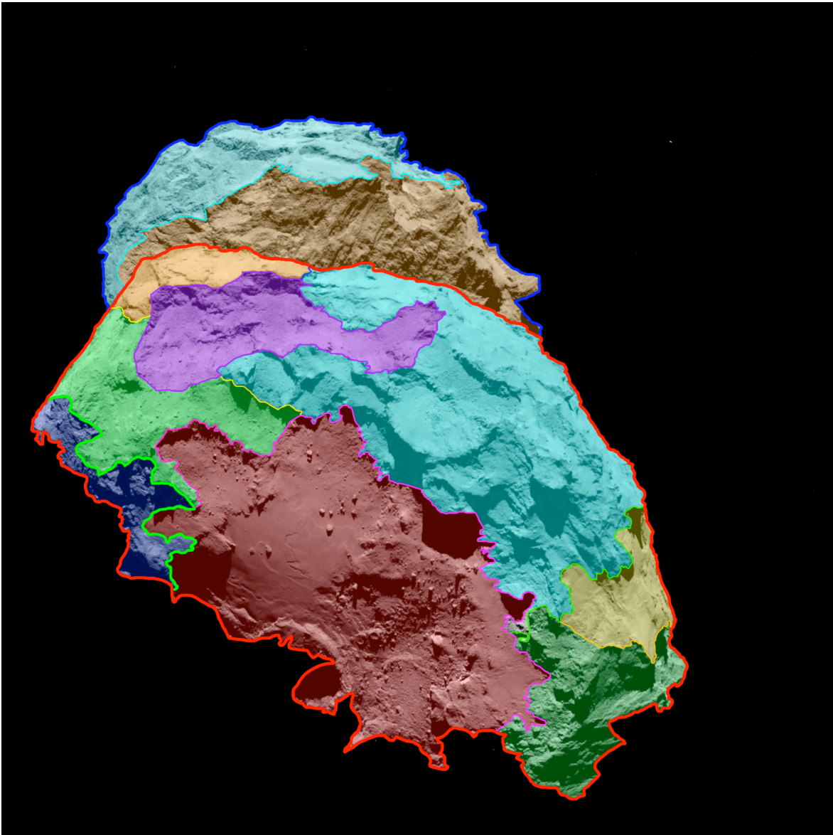
Figure 1: In this view of the “belly” and part of the “head” of comet 67P/Churyumov-Gerasimenko, several morphologically different regions are indicated. Credits: ESA/Rosetta/MPS for OSIRIS Team MPS/UPD/LAM/IAA/SSO/INTA/UPM/DASP/IDA
